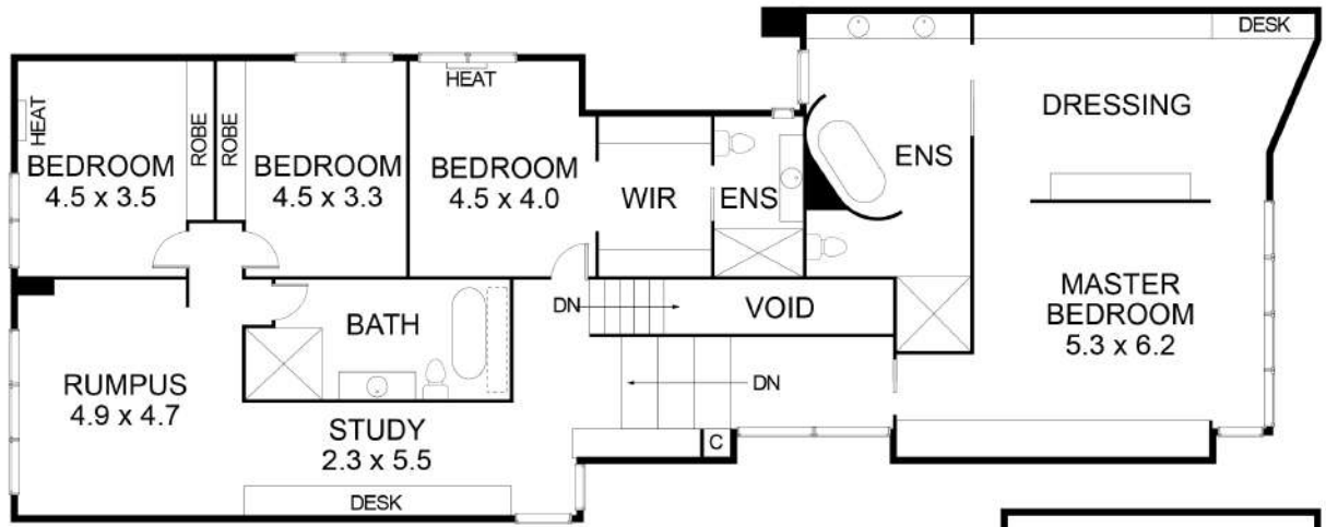
FIRST FLOOR
